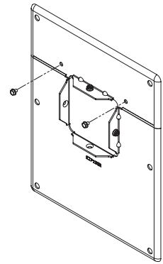
Use (2) #8-32 x 1/4" screws to secure plate sections together
