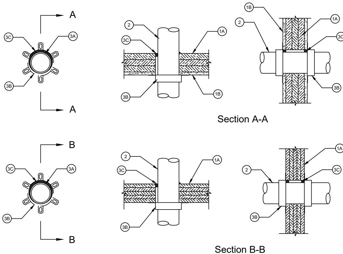
Figure 1. Through Penetration Detail
